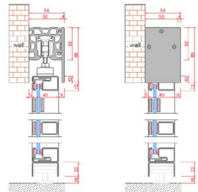
Wandmontage (System STANDARD)
